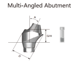
Screw Retained Restoration
