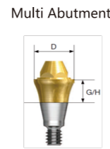
Screw Retained Restoration
